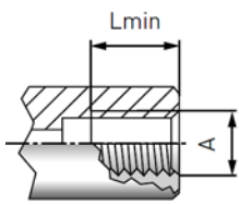
NPT 螺纹 (ANSI/ASME B1.20.1-1983)
