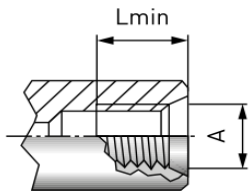
BSPT (锥形管螺纹)
